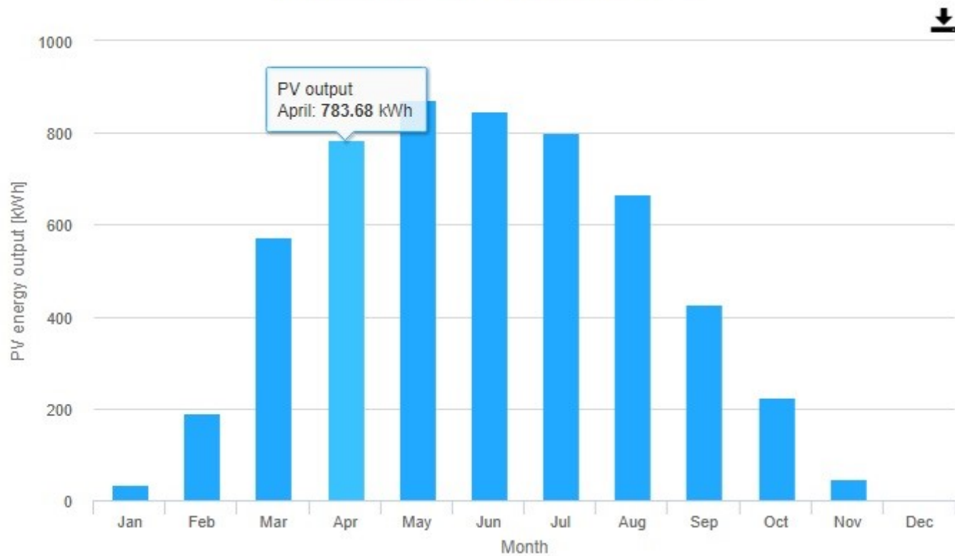
Monthly energy output from fix-angle PV system
